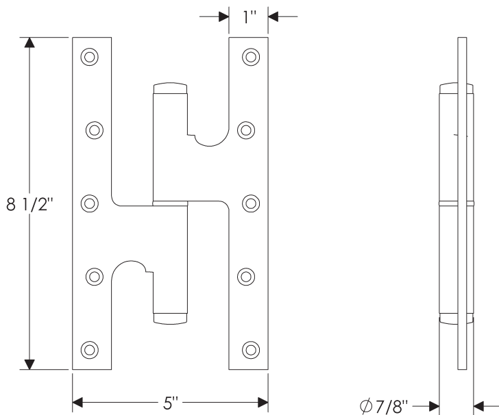
PHNG8.5x5 Paumelle Hinge 8 1/2" x 5"
