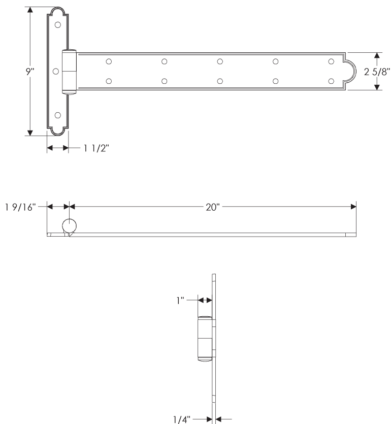
SHNG20 Strap Hinge 20"
