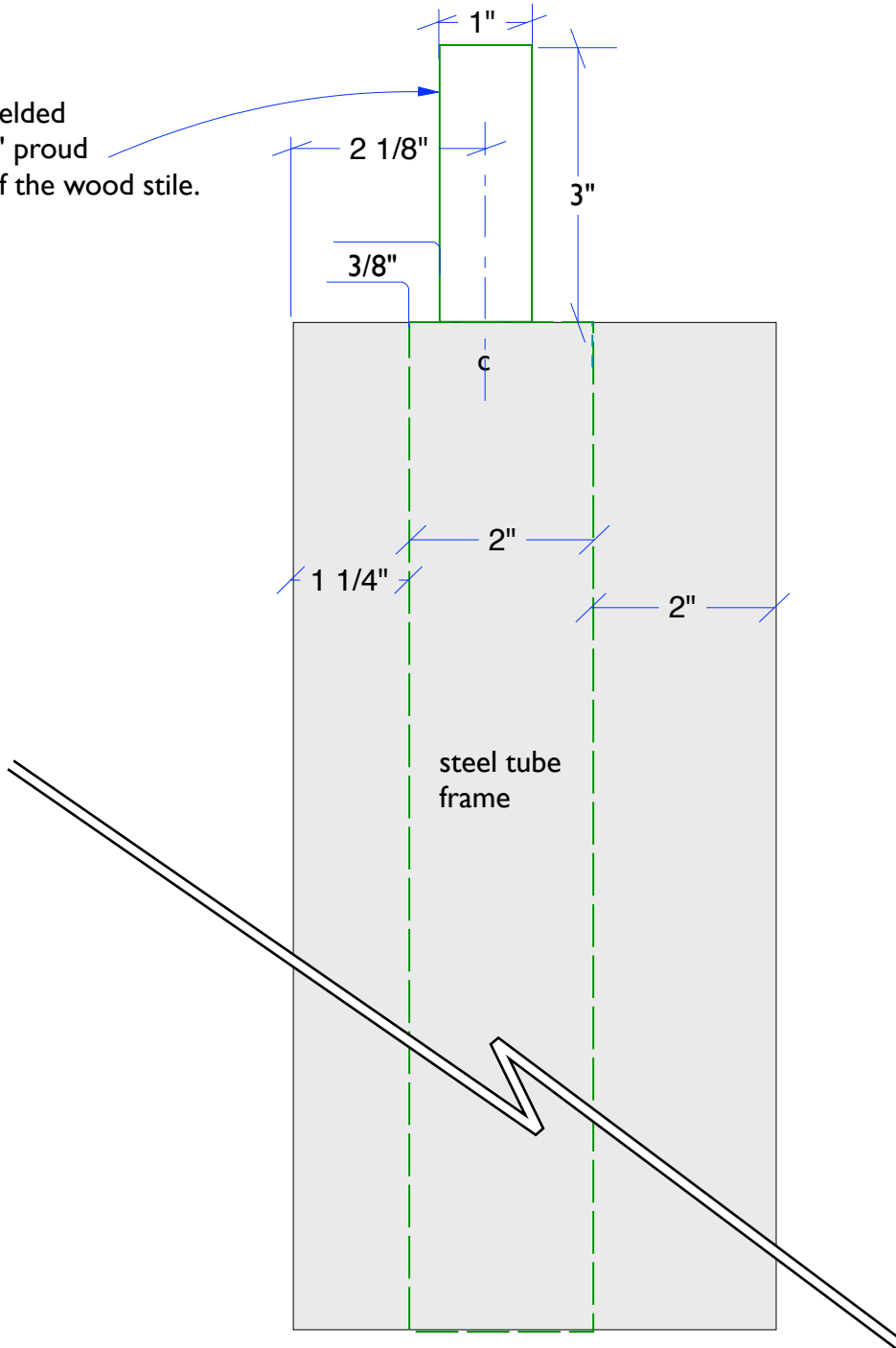
Left Gate Stile Profile
