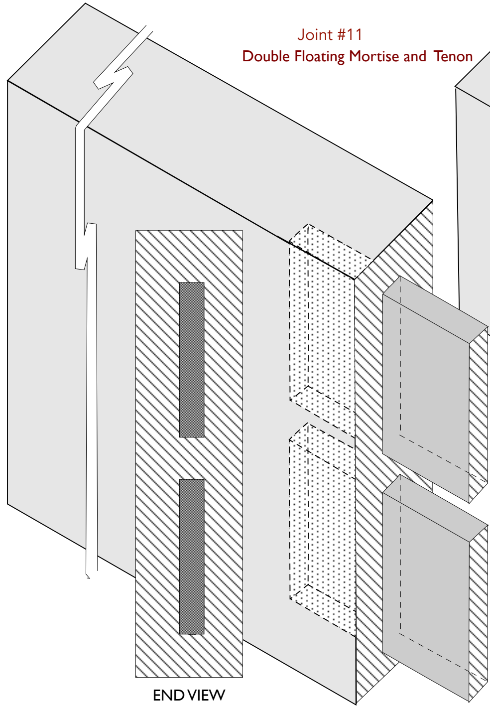
Floating Tenons
