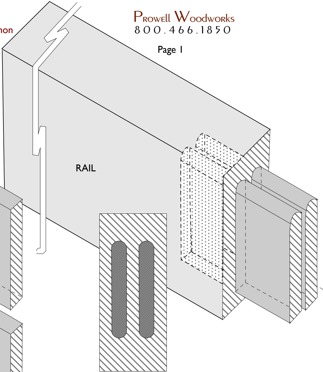
END VIEW
